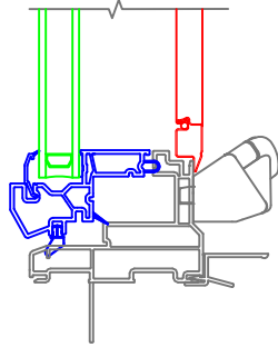
Without J-Channel 1/2"-5/8" Drywall Return
