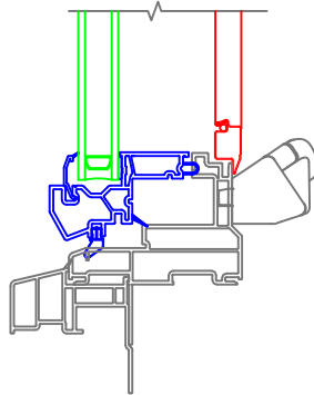
4-1/2 Banded Casing without J-Channel Standard Sill Nose
