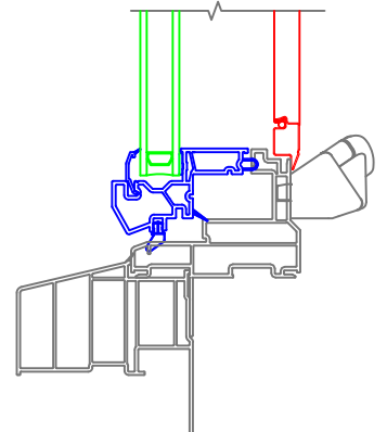
4-1/2 Banded Casing without J-Channel Historical Sill Nose
