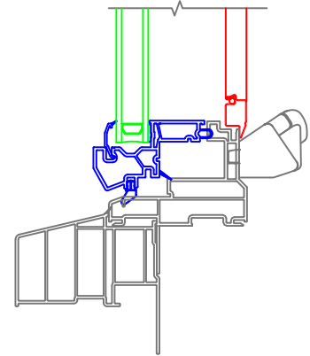
5/4 x 3-1/2 Flat Casing without J-Channel Historical Sill Nose
