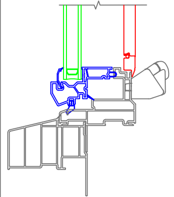
Brickmould Casing without J-Channel Historical Sill Nose
