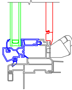
3/4" Drywall Return
