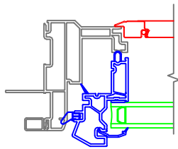
With Applied J-Channel
