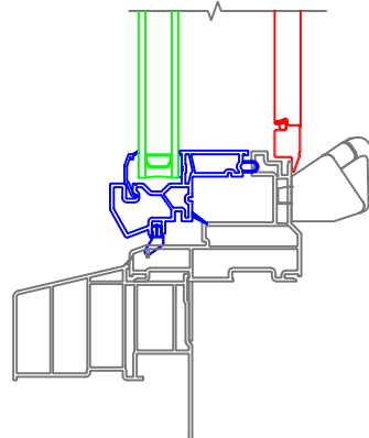
4-1/2 Banded Casing with J-Channel Historical Sill Nose
