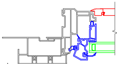
5/4 x 3-1/2 Flat Casing without J-Channel Standard Sill Nose
