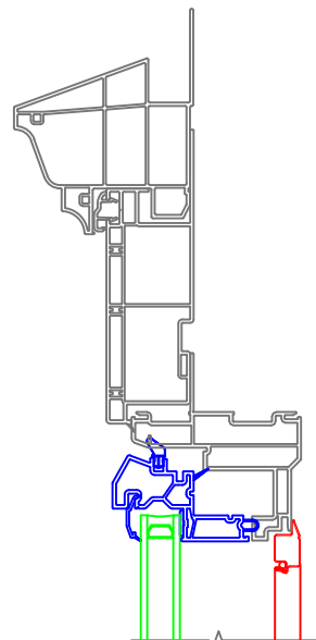
4-1/2 Banded Casing and Crown Crosshead Moulding
