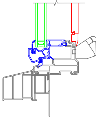
Brickmould Casing with J-Channel Historical Sill Nose
