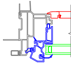
3/4" Drywall Return
