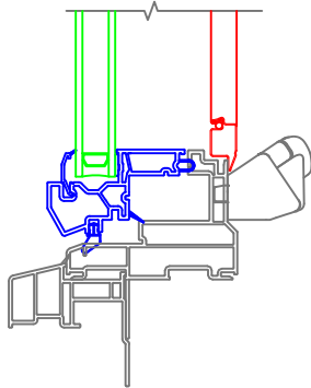
4-1/2 Banded Casing with J-Channel Standard Sill Nose
