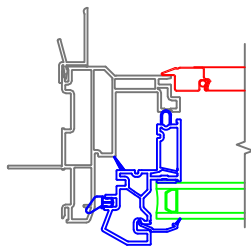
Without J-Channel
