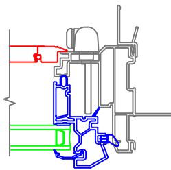
1/2"-5/8" Drywall Return
