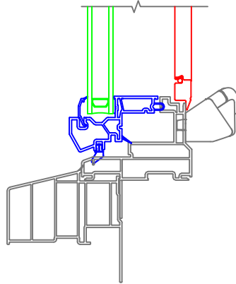
5/4 x 3-1/2 Flat Casing with J-Channel Historical Sill Nose
